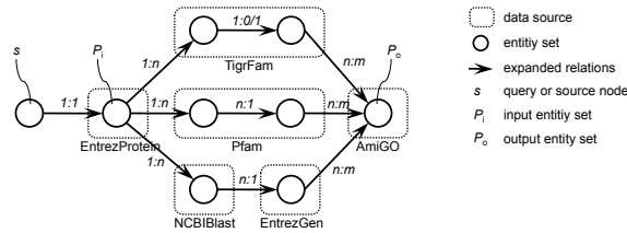
Figure 1: The subset of the E/R schema relevant to the exploratory query ( EntrezProtein.name = “ABCC8”, AmiGO ).
