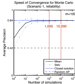
Figure 7: Effect of number of trials in the Monte Carlo algorithm on reliability ranking performance. 1000 trials already deliver very reliable results.
